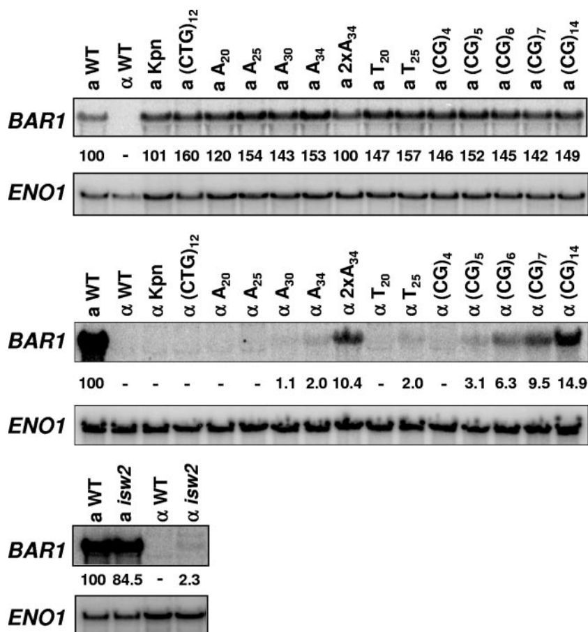
FIG. 4. Northern blot analysis of BARI . Strains analyzed are indicated above each lane. The designations of strains are described in the legend of Fig. 2, except for (CG)_{14} , which refers to (CG)_7 TATA (CG)_7 inserted into the BARI promoter. Northern blots were probed with the BARI probe and then stripped and reprobed with the ENO1 probe as a loading control, which is not regulated by mating type. The BARI mRNA levels, which are shown under the BARI blot, were determined as the BARI / ENO1 ratio by using a phosphorimager and were normalized to the intensity of the MATa WT strain, set as 100. These normalized ratios are shown at the bottom of the BARI blot.
